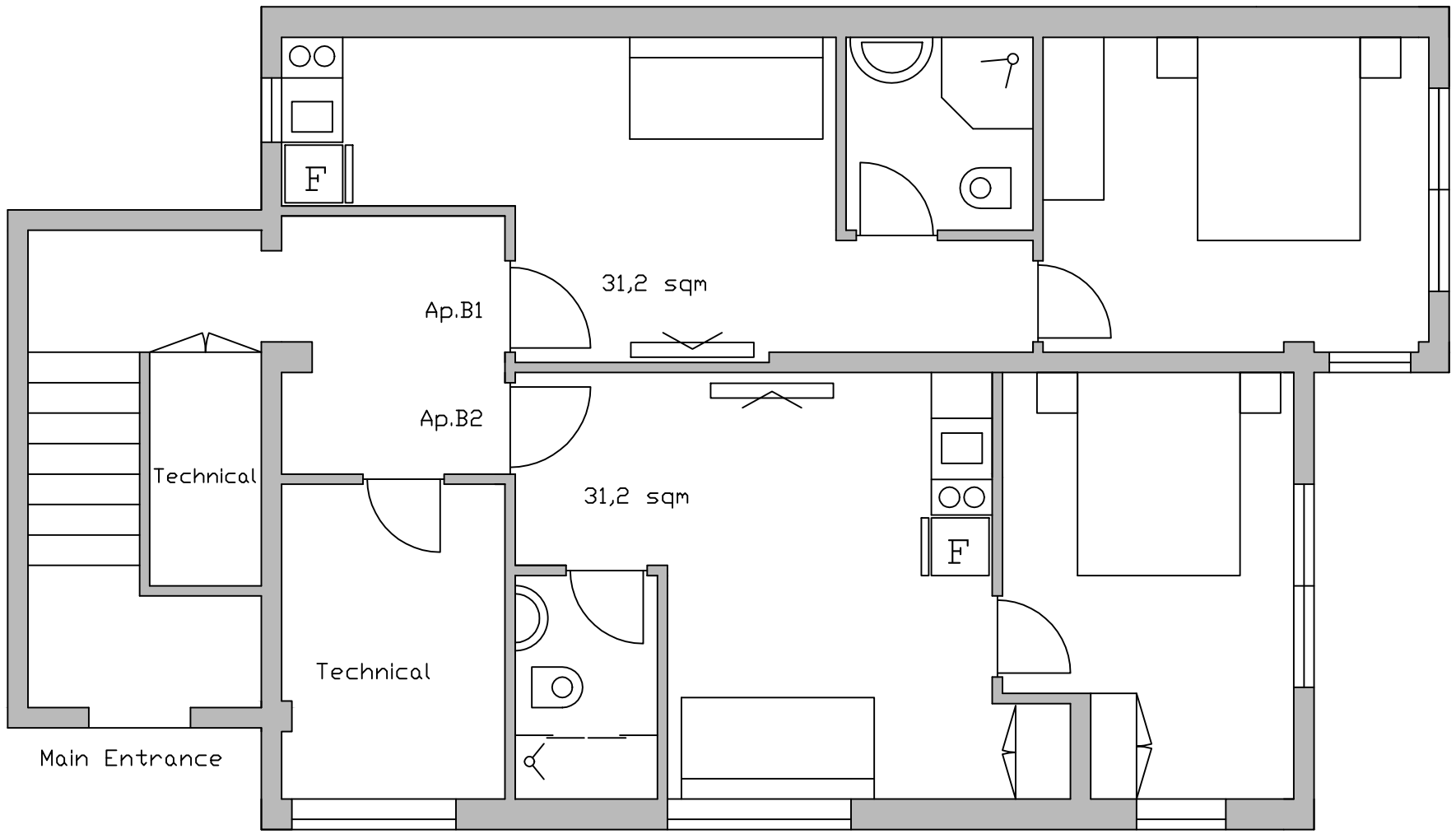
GROUND FLOOR
